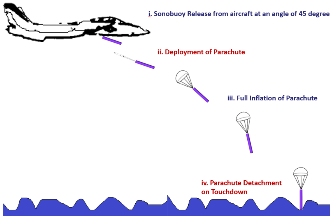
Fig: Sequence of Operation
